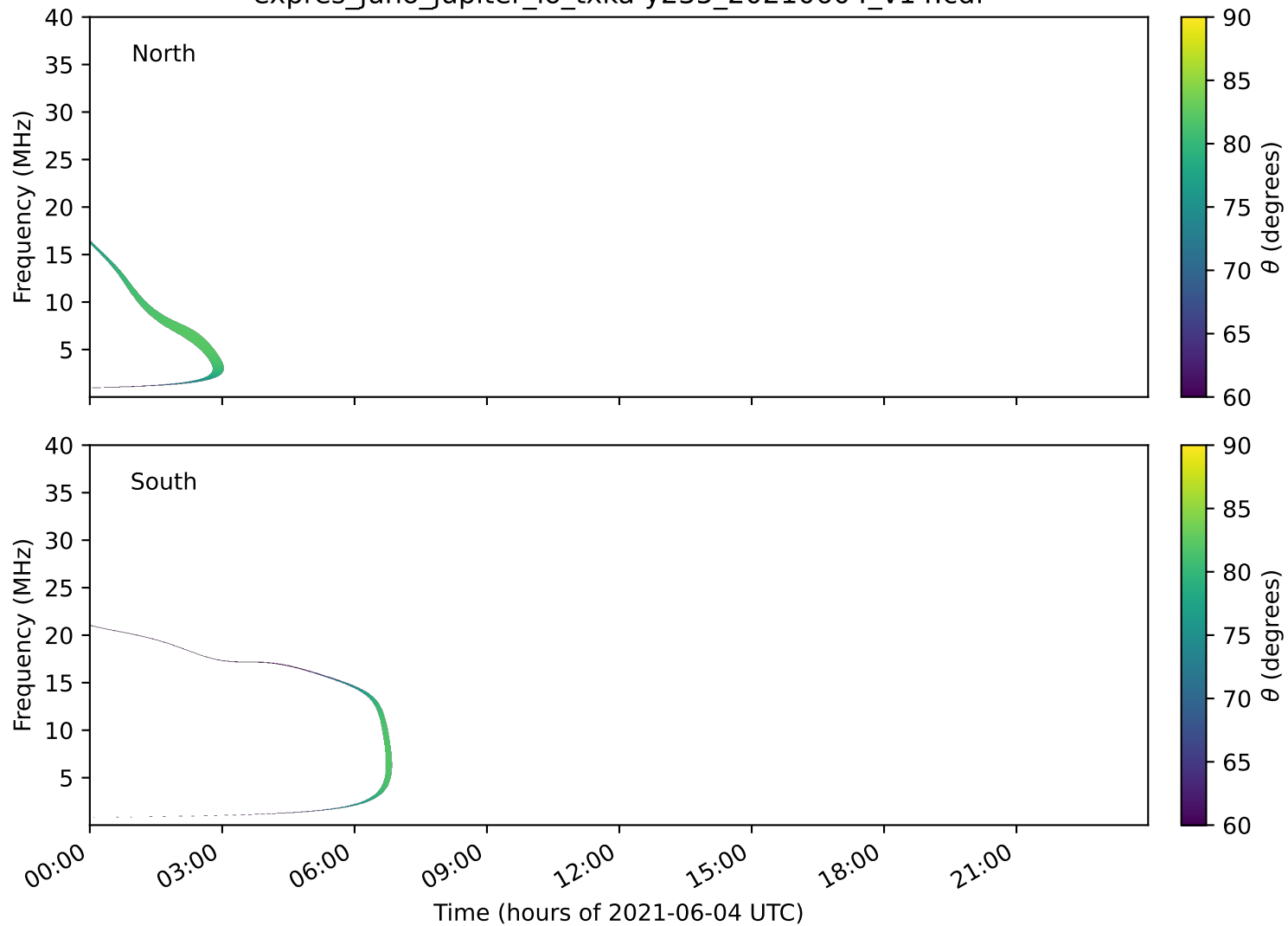
expres_juno_jupiter_io_txka-y235_20210604_v14.cdf
