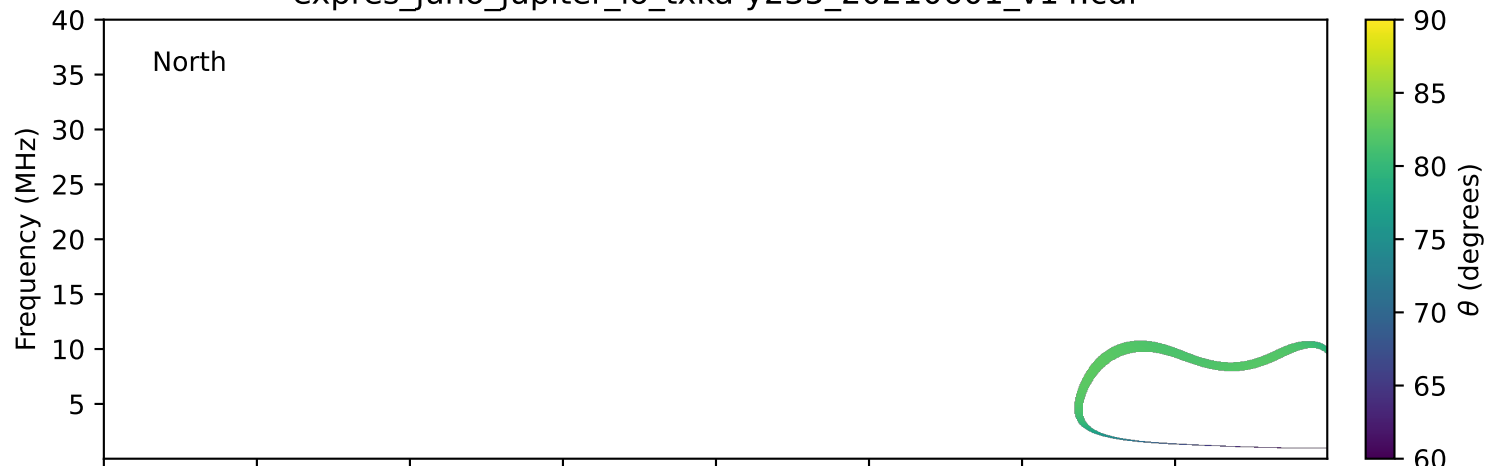
expres_juno_jupiter_io_txka-y235_20210601_v14.cdf
