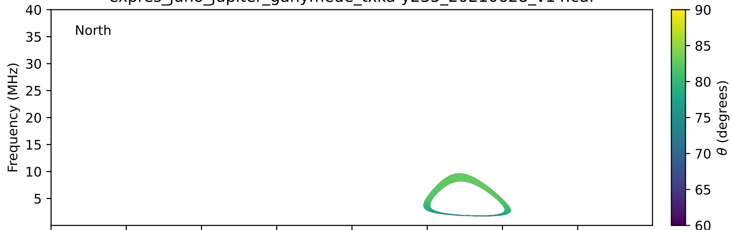
expres_juno_jupiter_ganymede_txka-y235_20210628_v14.cdf
