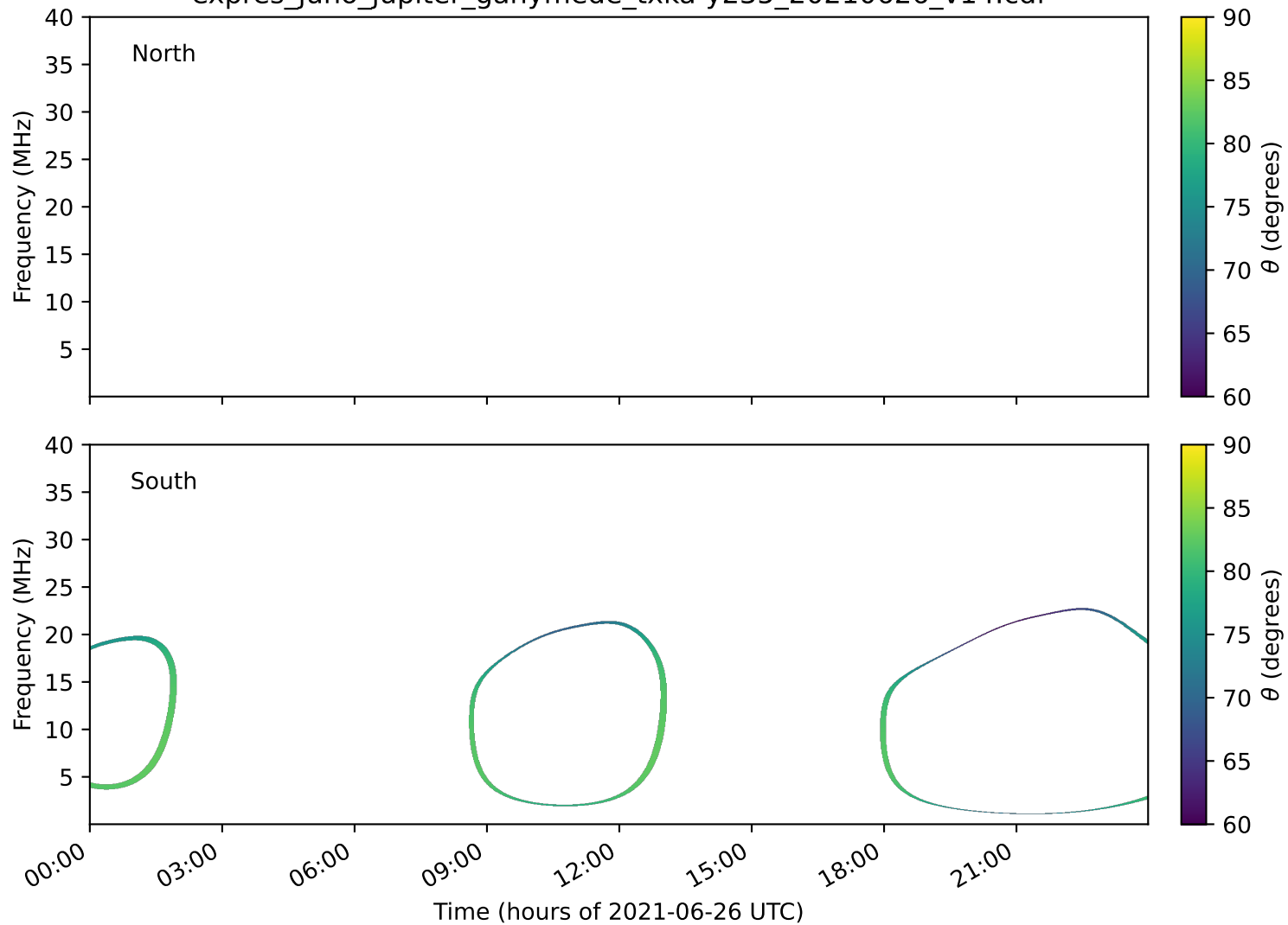
expres_juno_jupiter_ganymede_txka-y235_20210626_v14.cdf
