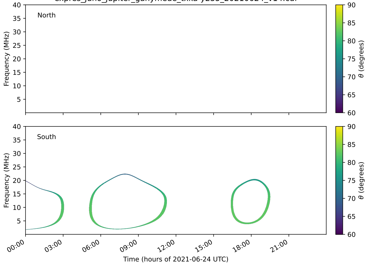
expres_juno_jupiter_ganymede_txka-y235_20210624_v14.cdf
