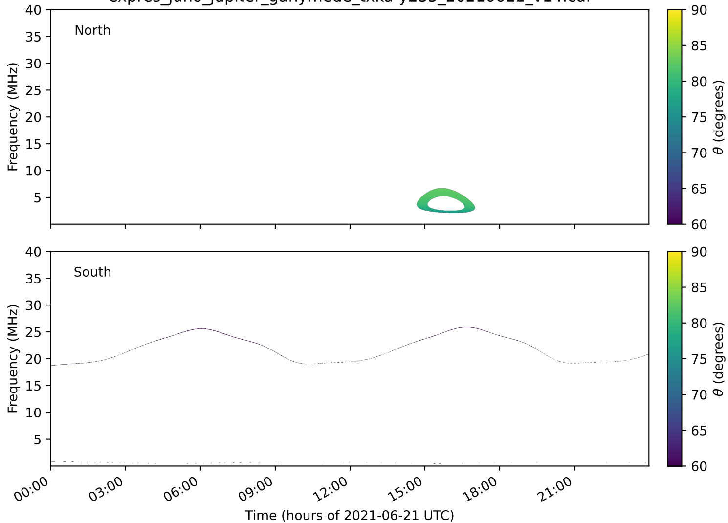
expres_juno_jupiter_ganymede_txka-y235_20210621_v14.cdf
