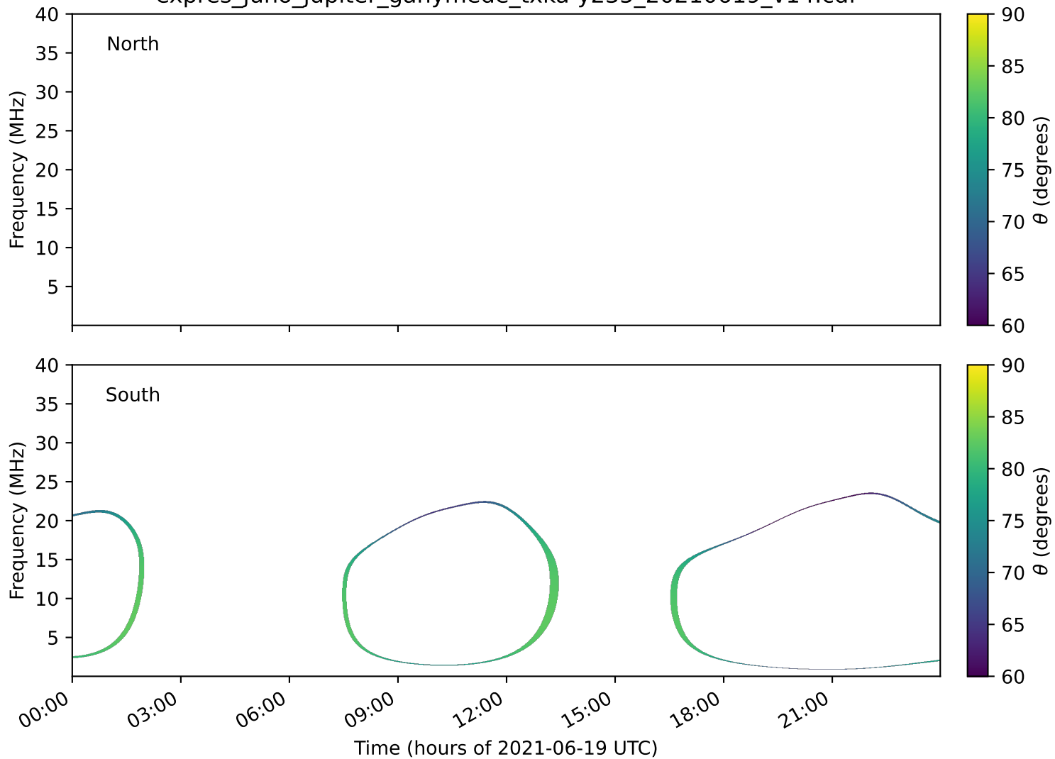
expres_juno_jupiter_ganymede_txka-y235_20210619_v14.cdf
