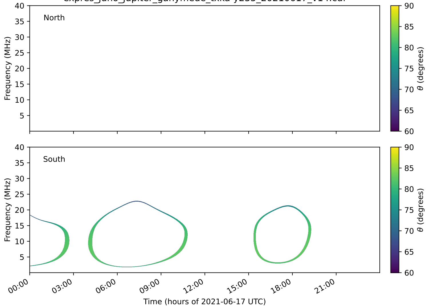
expres_juno_jupiter_ganymede_txka-y235_20210617_v14.cdf
