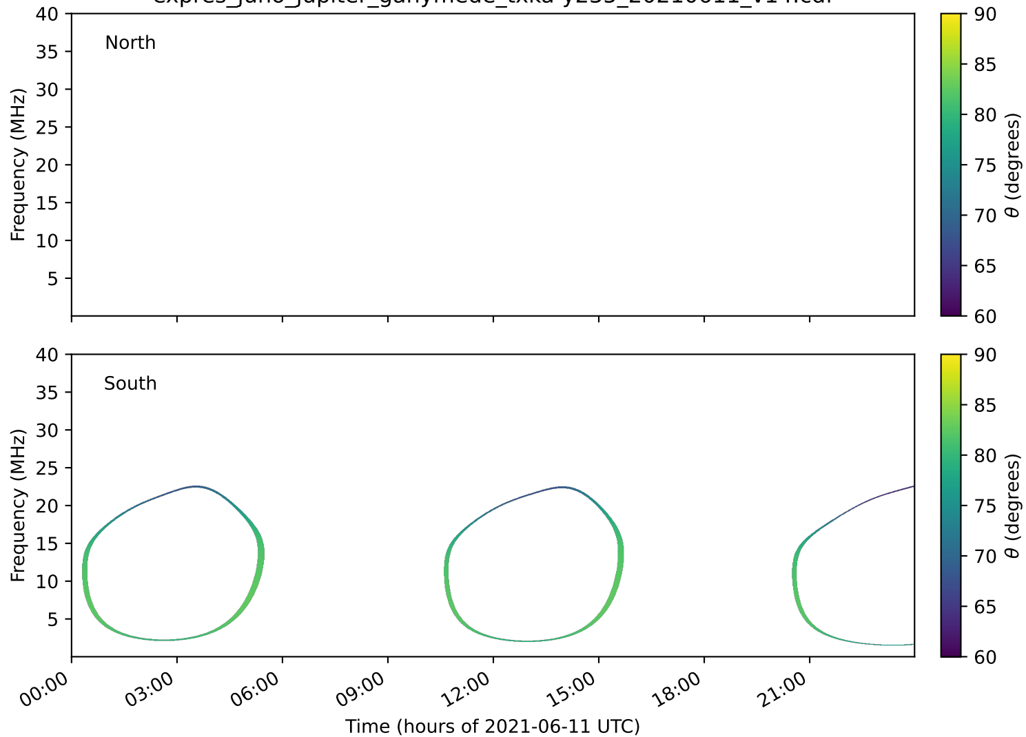
expres_juno_jupiter_ganymede_txka-y235_20210611_v14.cdf
