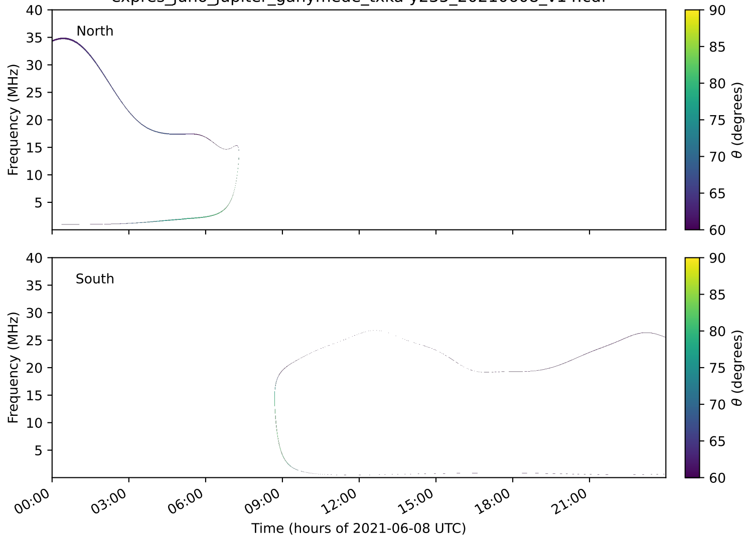
expres_juno_jupiter_ganymede_txka-y235_20210608_v14.cdf
