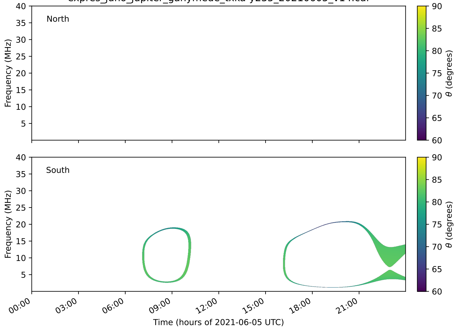
expres_juno_jupiter_ganymede_txka-y235_20210605_v14.cdf
