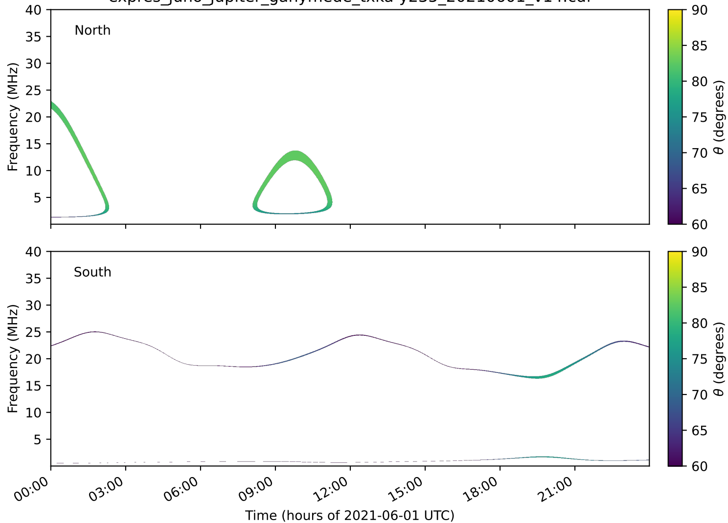
expres_juno_jupiter_ganymede_txka-y235_20210601_v14.cdf
