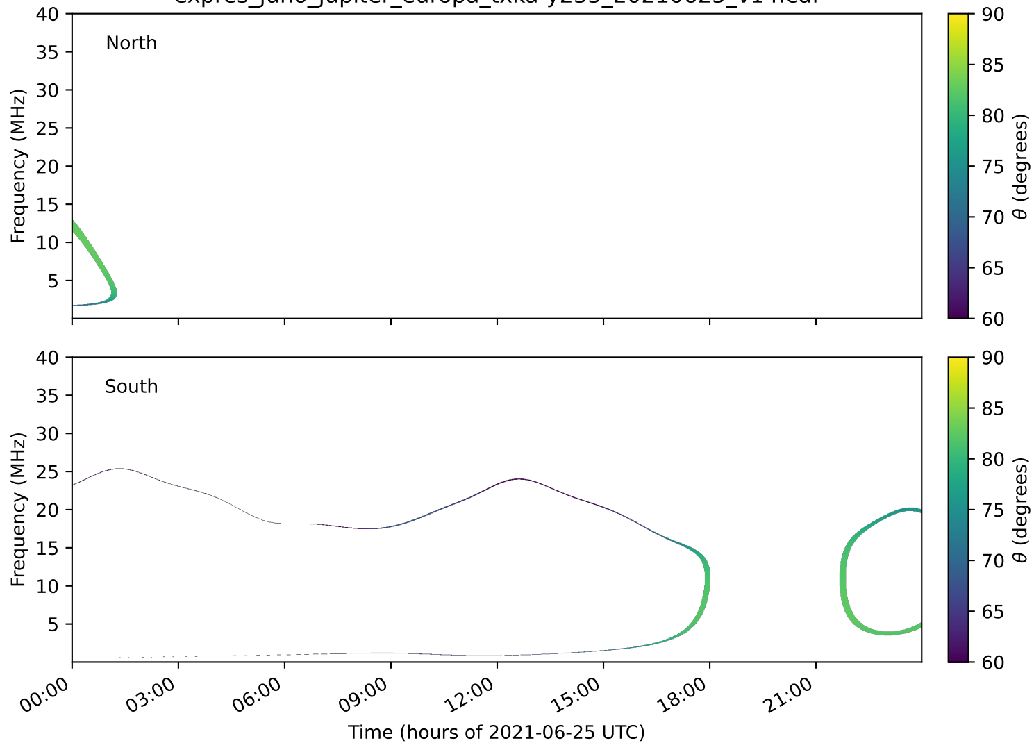
expres_juno_jupiter_europa_txka-y235_20210625_v14.cdf
