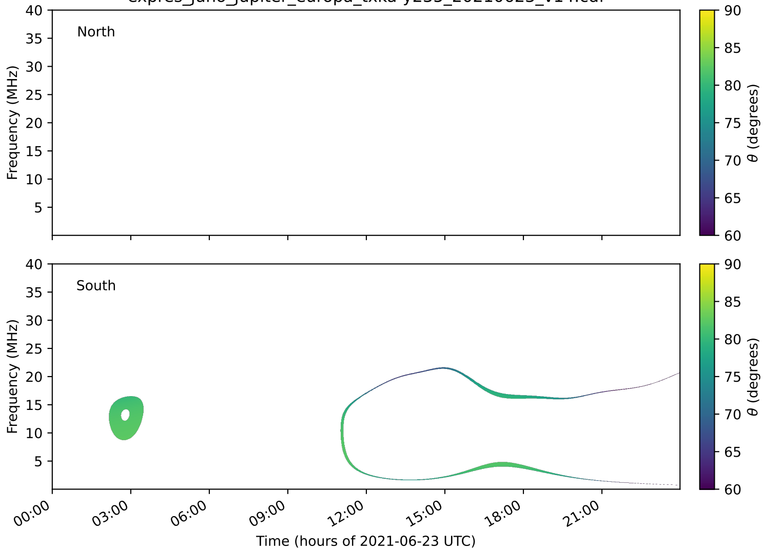
expres_juno_jupiter_europa_txka-y235_20210623_v14.cdf
