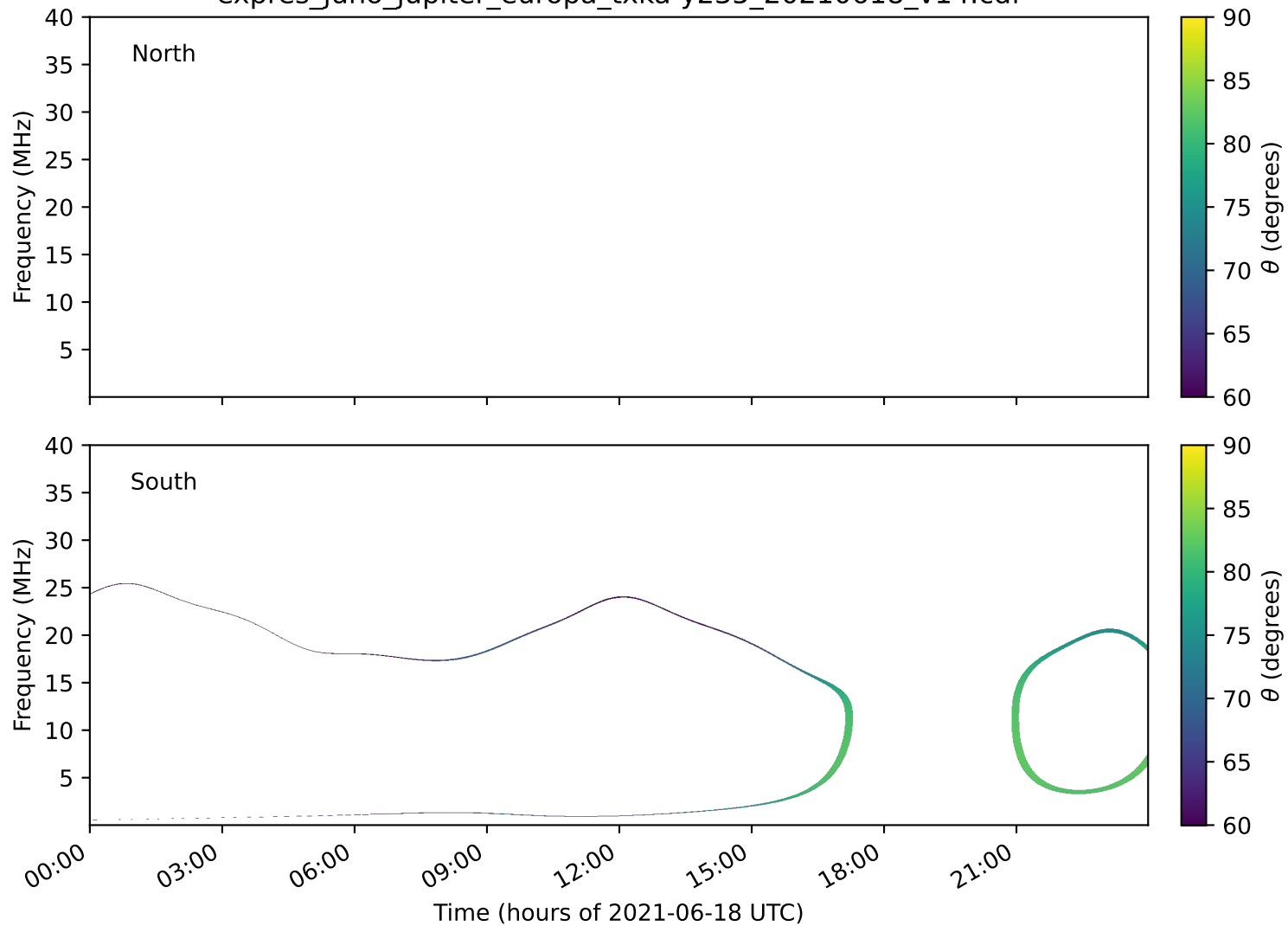
expres_juno_jupiter_europa_txka-y235_20210618_v14.cdf
