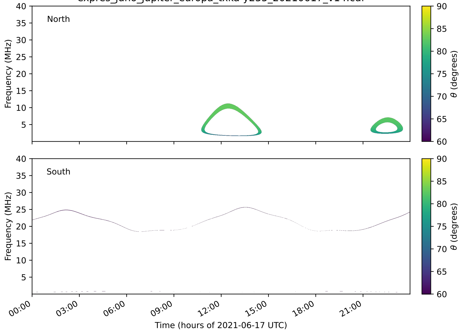
expres_juno_jupiter_europa_txka-y235_20210617_v14.cdf
