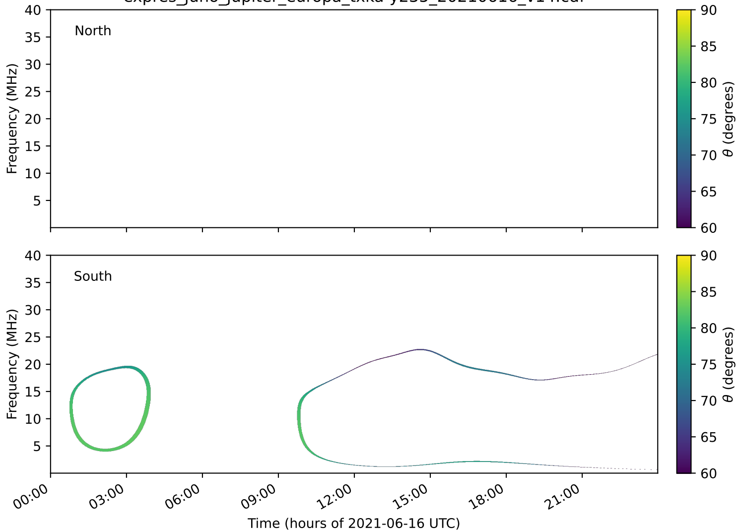
expres_juno_jupiter_europa_txka-y235_20210616_v14.cdf
