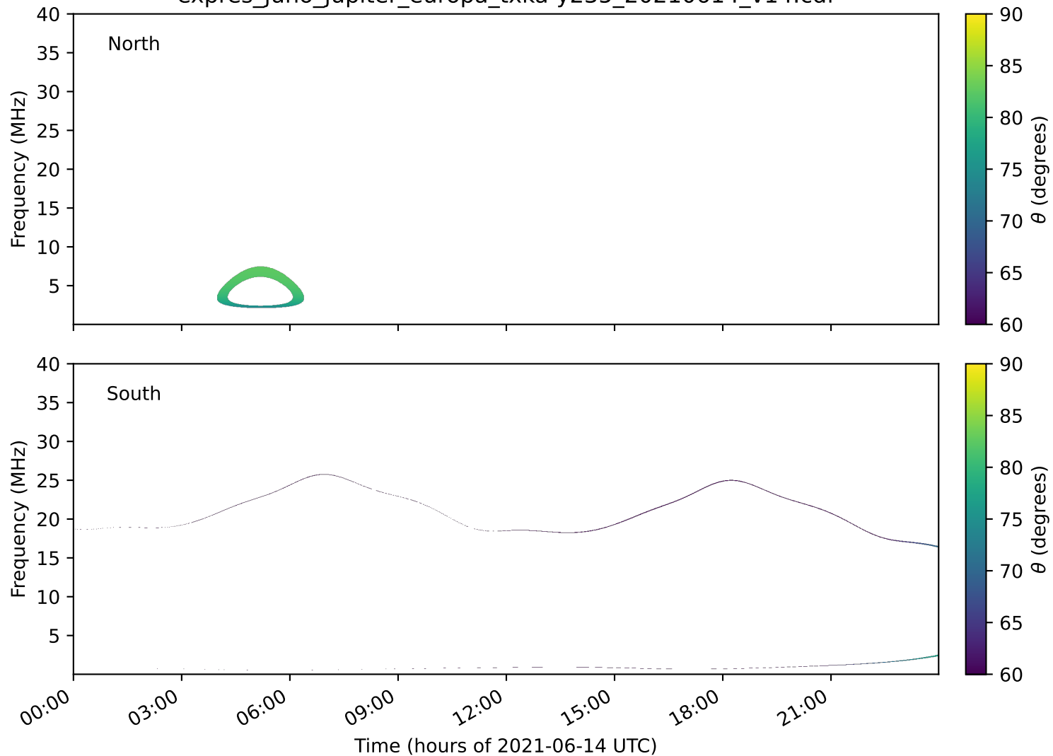
expres_juno_jupiter_europa_txka-y235_20210614_v14.cdf
