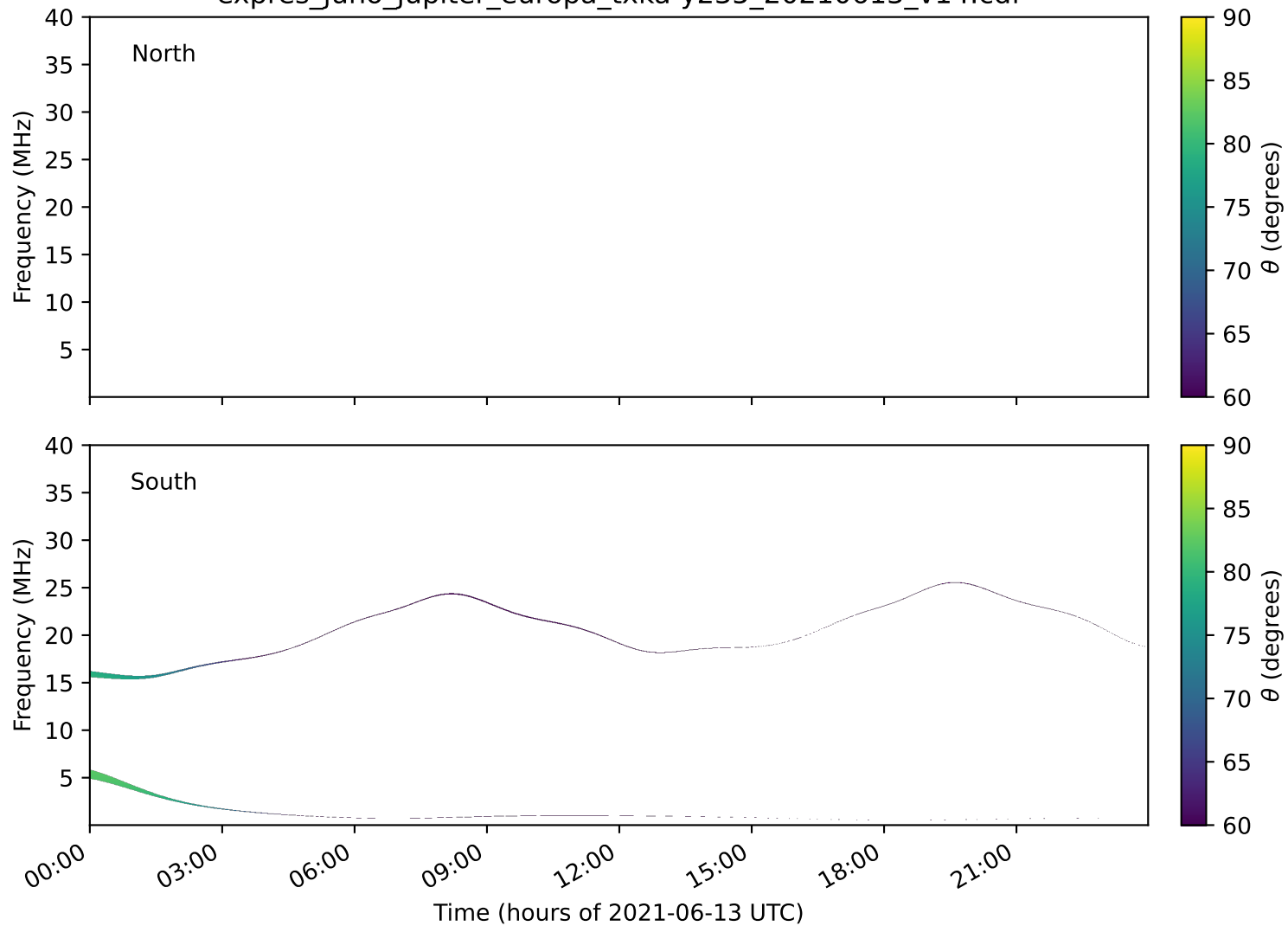
expres_juno_jupiter_europa_txka-y235_20210613_v14.cdf
