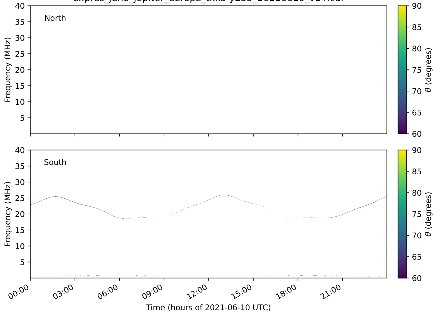
expres_juno_jupiter_europa_txka-y235_20210610_v14.cdf
