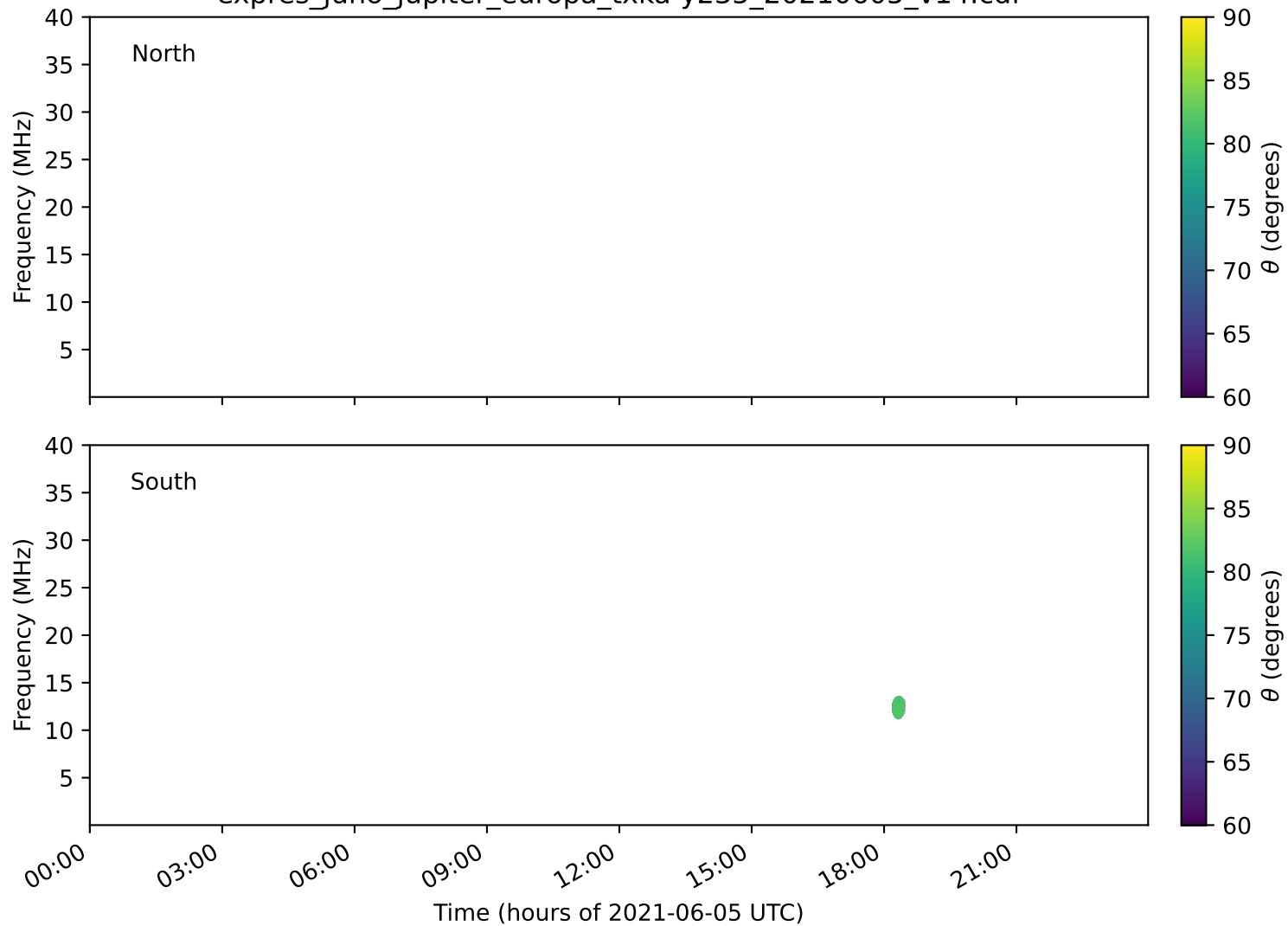
expres_juno_jupiter_europa_txka-y235_20210605_v14.cdf
