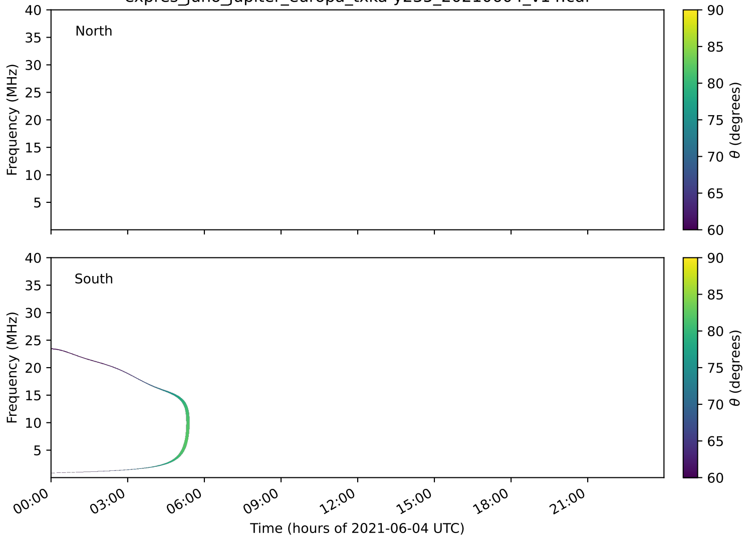
expres_juno_jupiter_europa_txka-y235_20210604_v14.cdf
