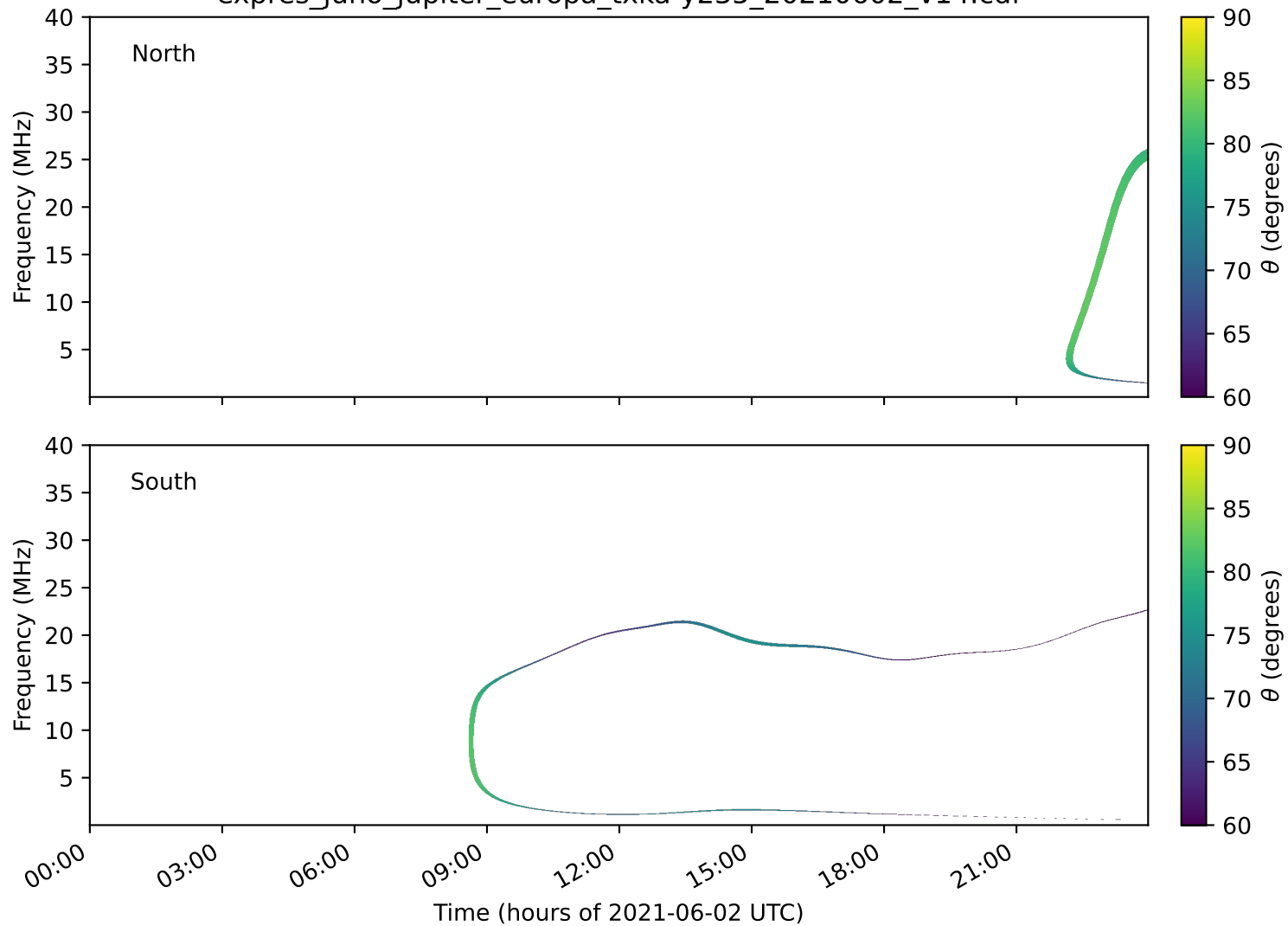
expres_juno_jupiter_europa_txka-y235_20210602_v14.cdf
