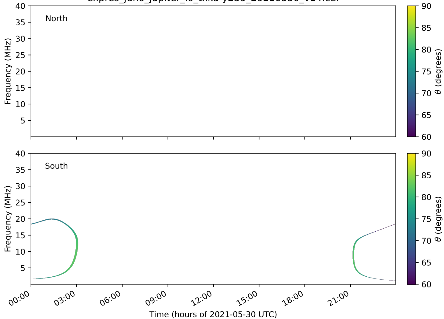
expres_juno_jupiter_io_txka-y235_20210530_v14.cdf
