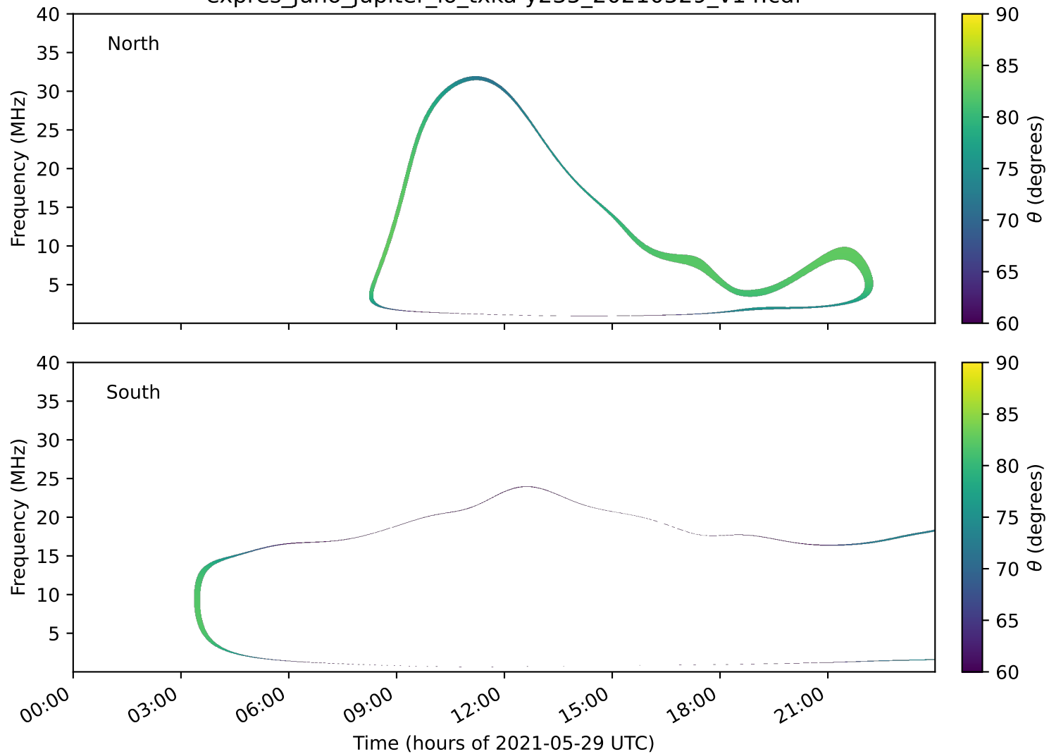
expres_juno_jupiter_io_txka-y235_20210529_v14.cdf
