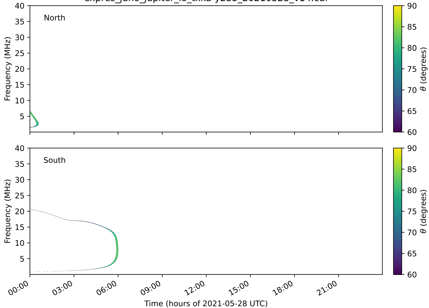
expres_juno_jupiter_io_txka-y235_20210528_v14.cdf
