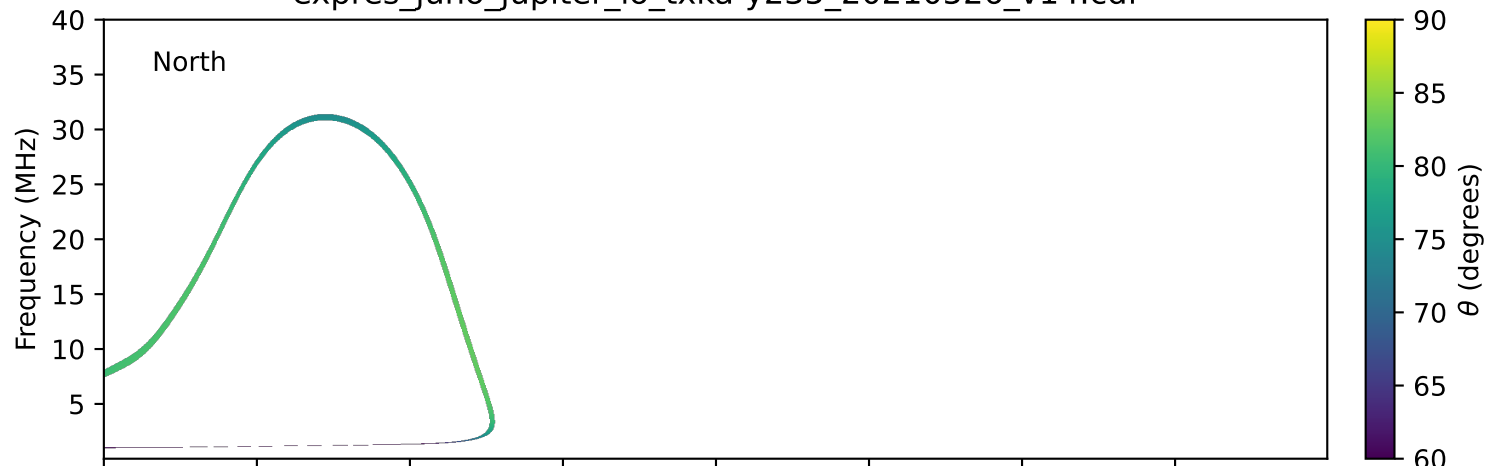
expres_juno_jupiter_io_txka-y235_20210526_v14.cdf
