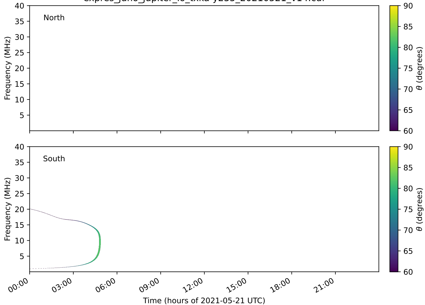
expres_juno_jupiter_io_txka-y235_20210521_v14.cdf
