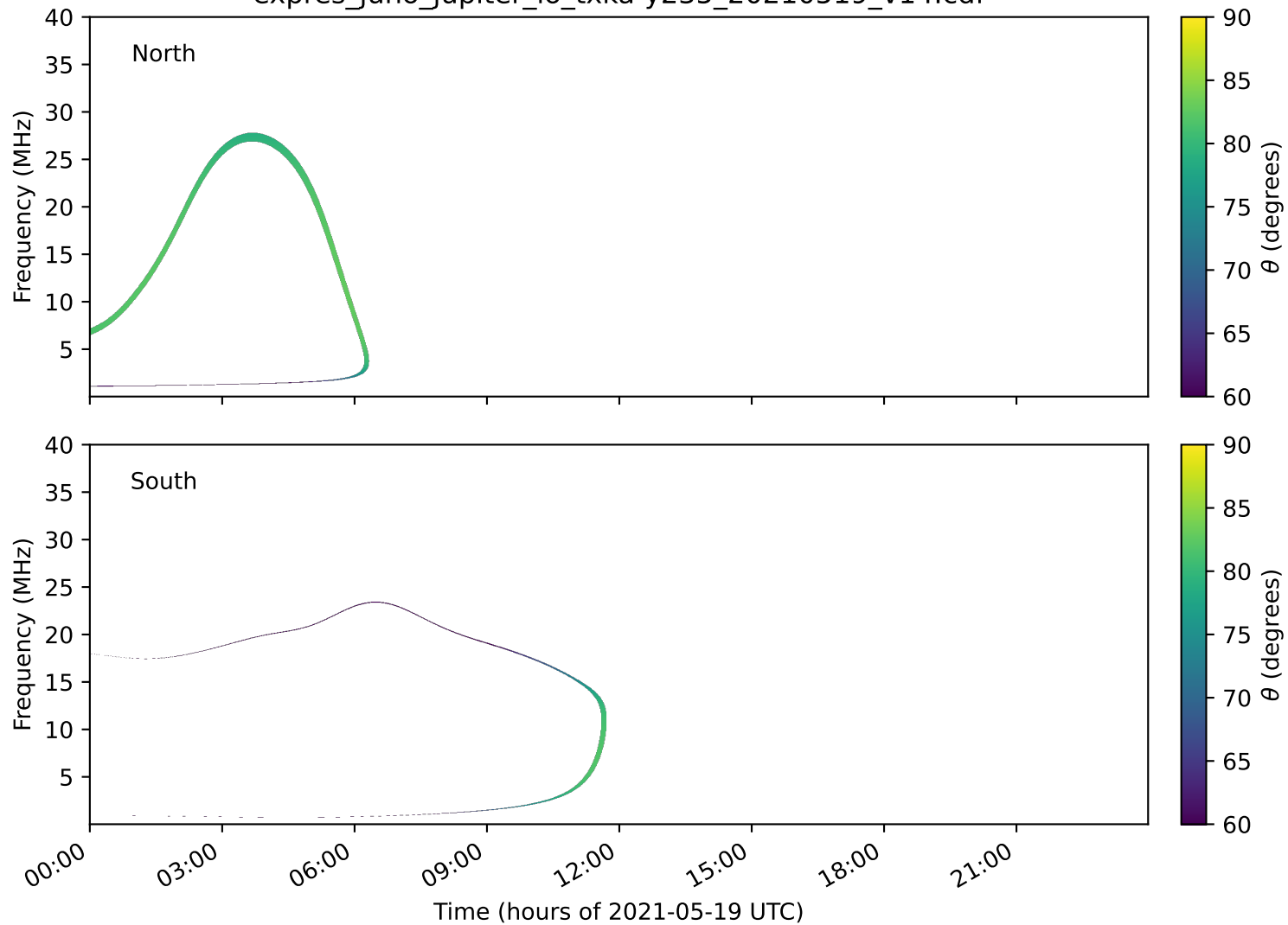
expres_juno_jupiter_io_txka-y235_20210519_v14.cdf
