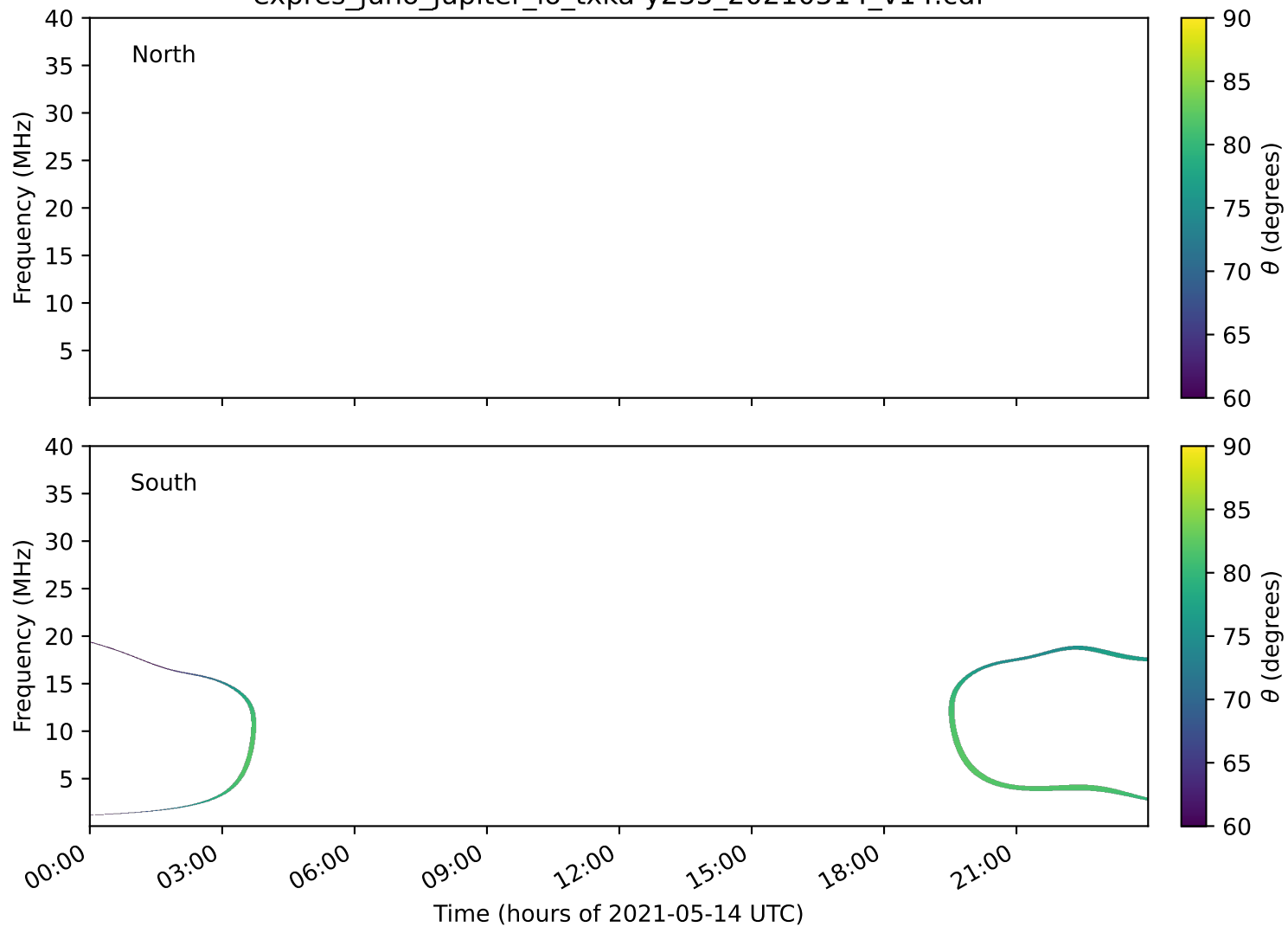
expres_juno_jupiter_io_txka-y235_20210514_v14.cdf
