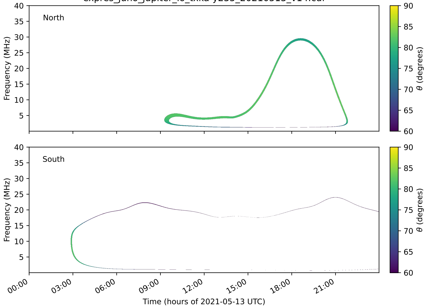
expres_juno_jupiter_io_txka-y235_20210513_v14.cdf
