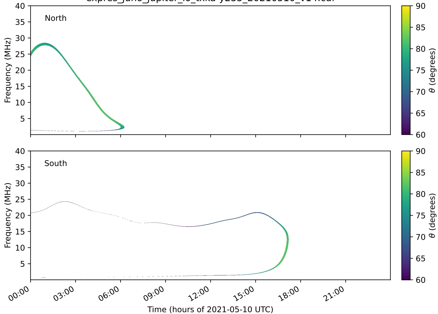
expres_juno_jupiter_io_txka-y235_20210510_v14.cdf
