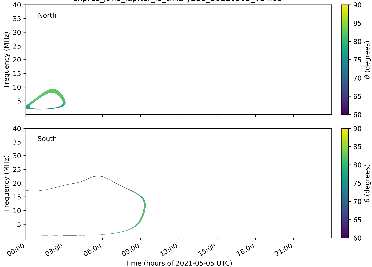
expres_juno_jupiter_io_txka-y235_20210505_v14.cdf
