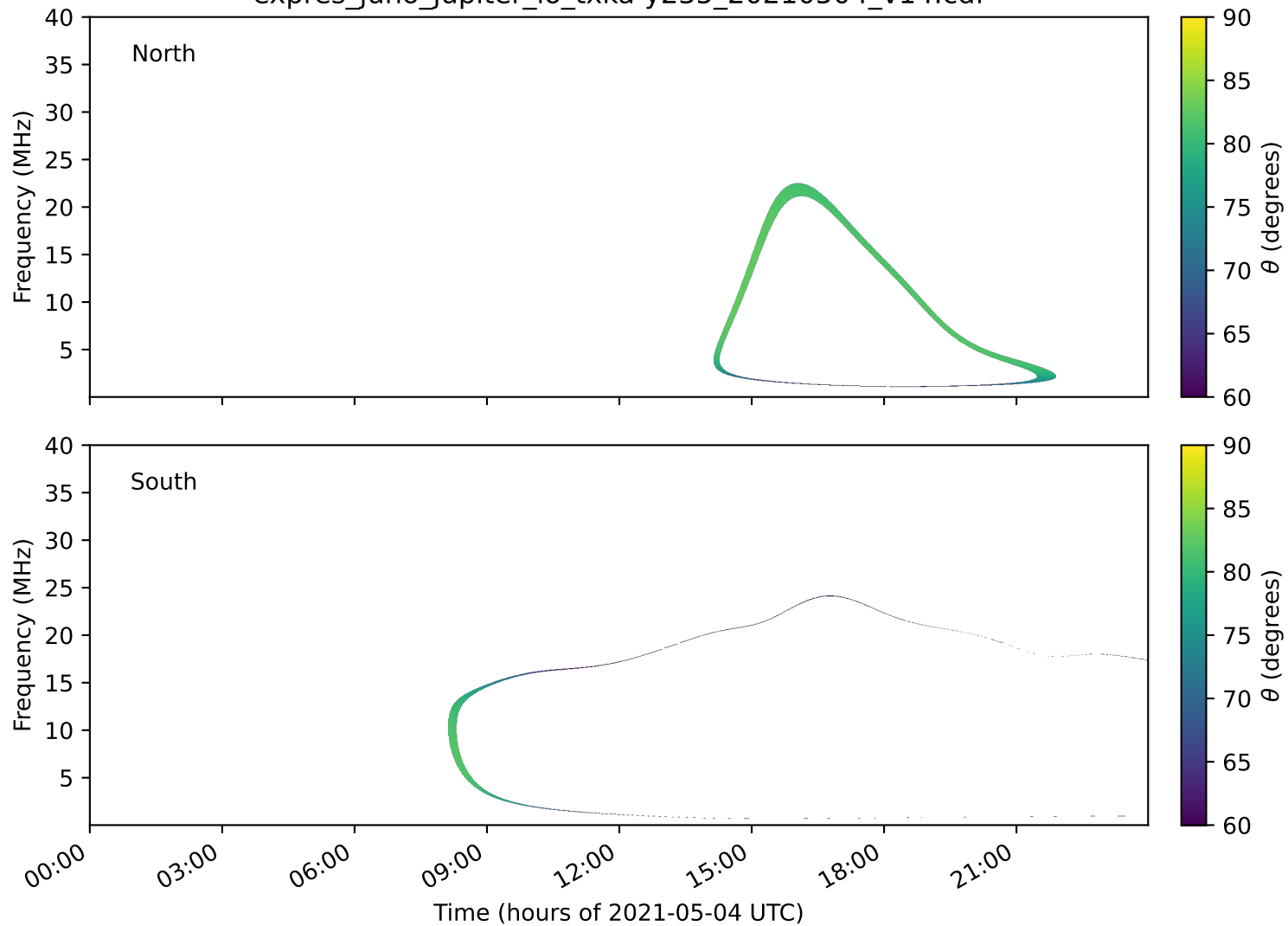
expres_juno_jupiter_io_txka-y235_20210504_v14.cdf
