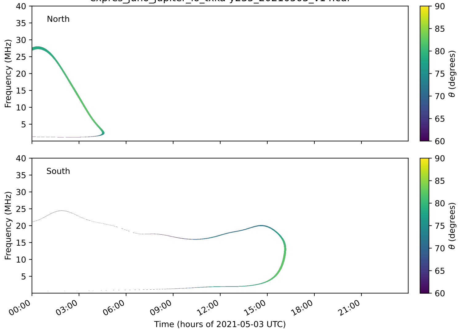
expres_juno_jupiter_io_txka-y235_20210503_v14.cdf
