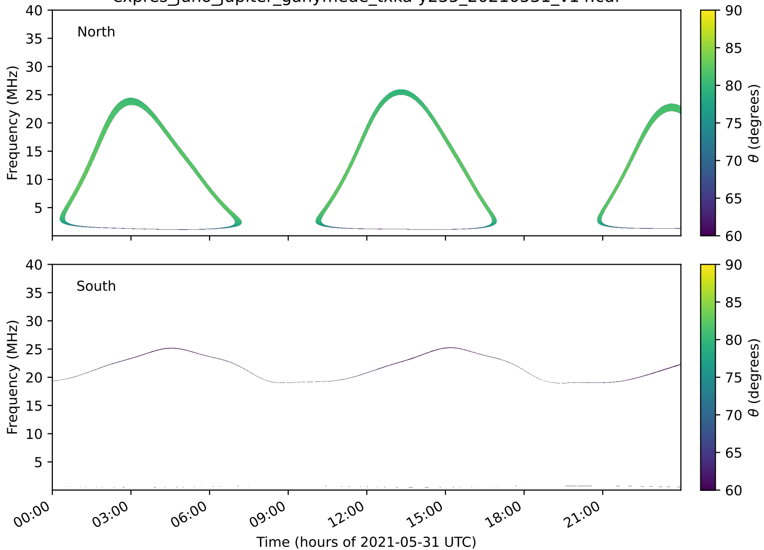
expres_juno_jupiter_ganymede_txka-y235_20210531_v14.cdf
