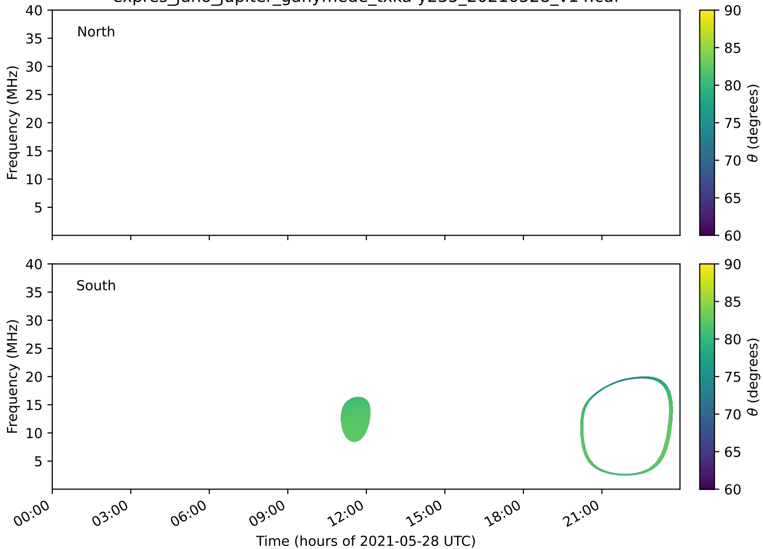
expres_juno_jupiter_ganymede_txka-y235_20210528_v14.cdf
