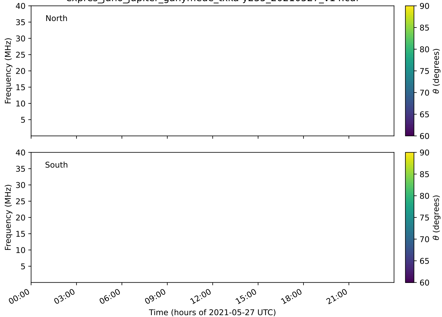
expres_juno_jupiter_ganymede_txka-y235_20210527_v14.cdf
