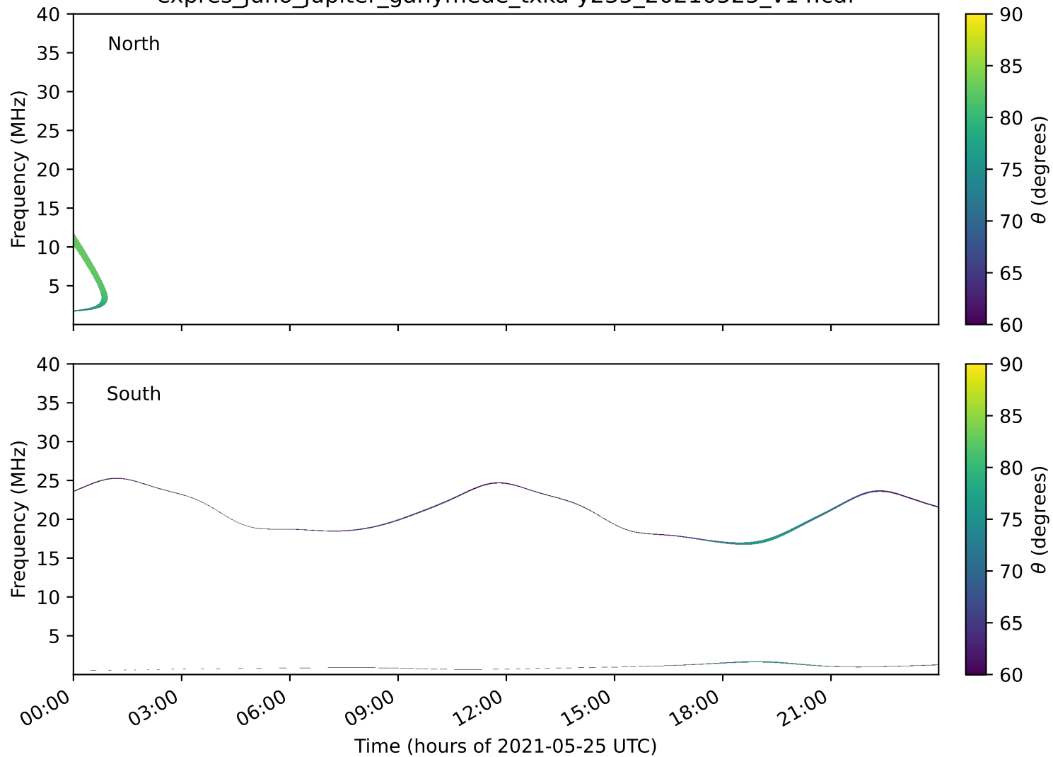
expres_juno_jupiter_ganymede_txka-y235_20210525_v14.cdf
