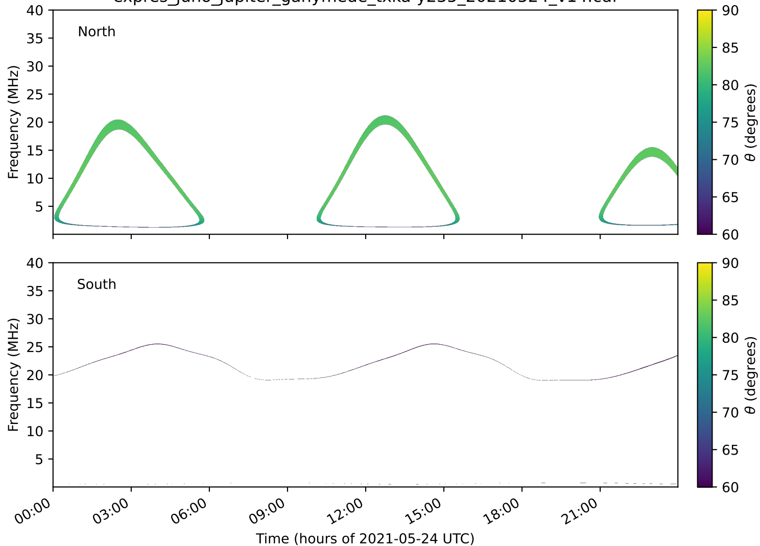
expres_juno_jupiter_ganymede_txka-y235_20210524_v14.cdf
