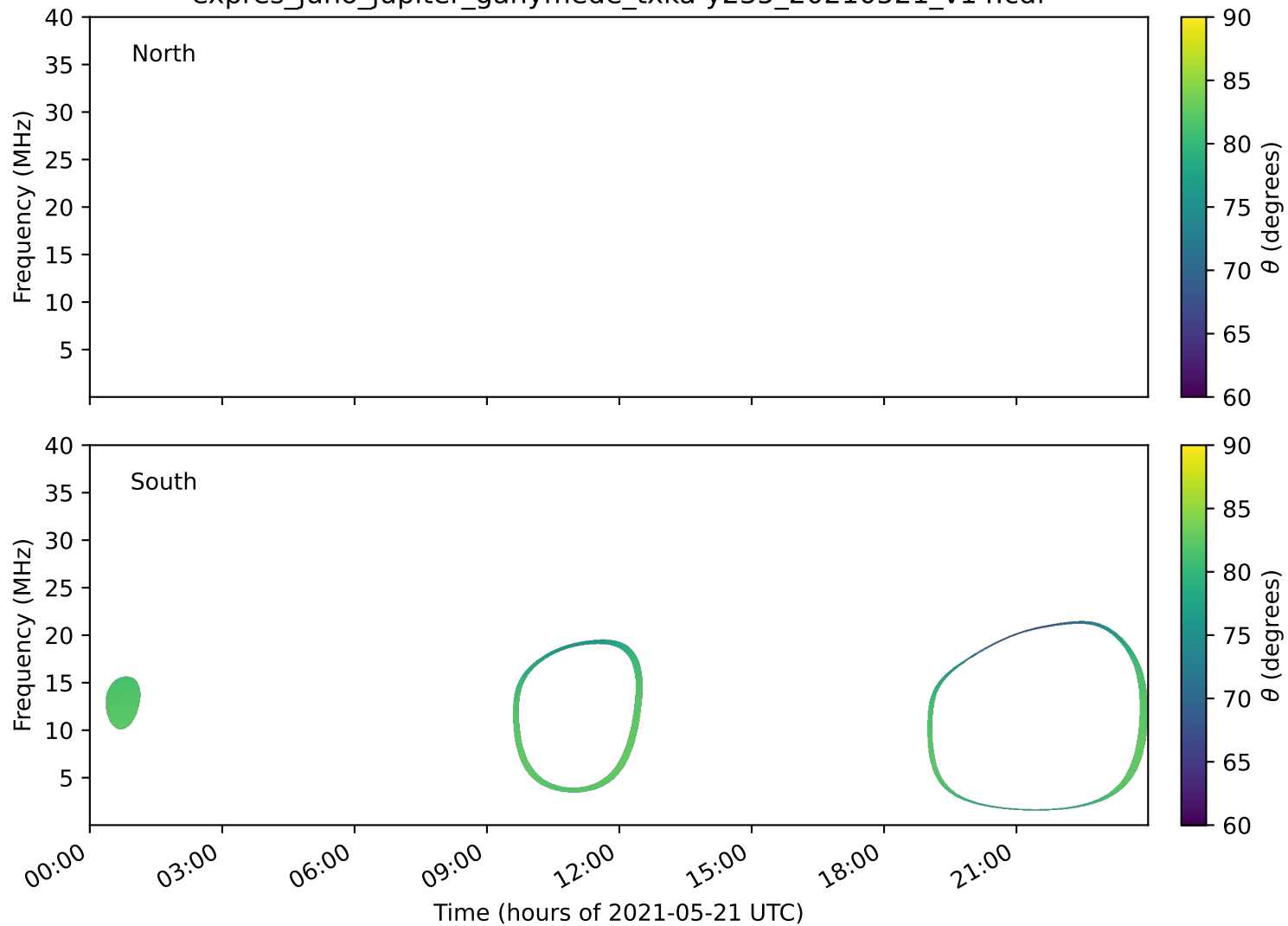
expres_juno_jupiter_ganymede_txka-y235_20210521_v14.cdf
