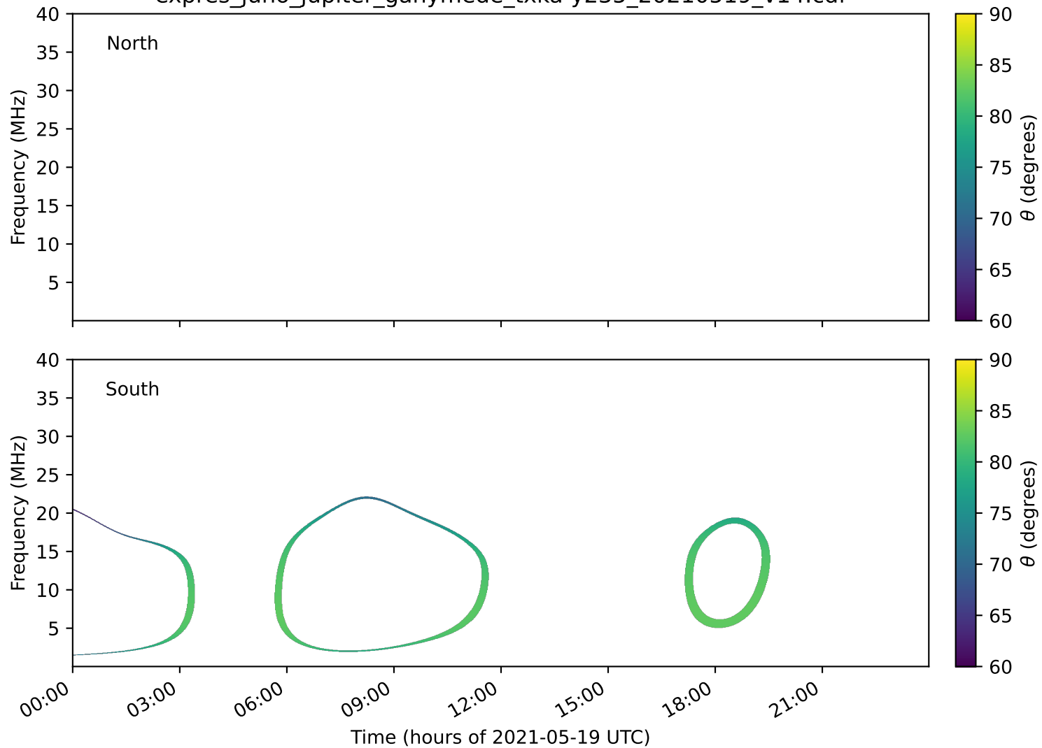
expres_juno_jupiter_ganymede_txka-y235_20210519_v14.cdf
