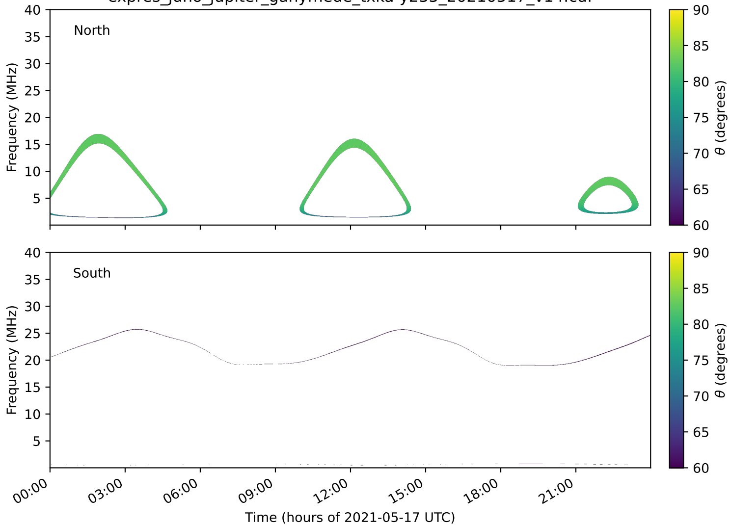
expres_juno_jupiter_ganymede_txka-y235_20210517_v14.cdf
