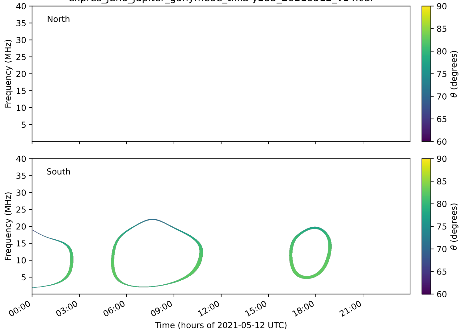
expres_juno_jupiter_ganymede_txka-y235_20210512_v14.cdf
