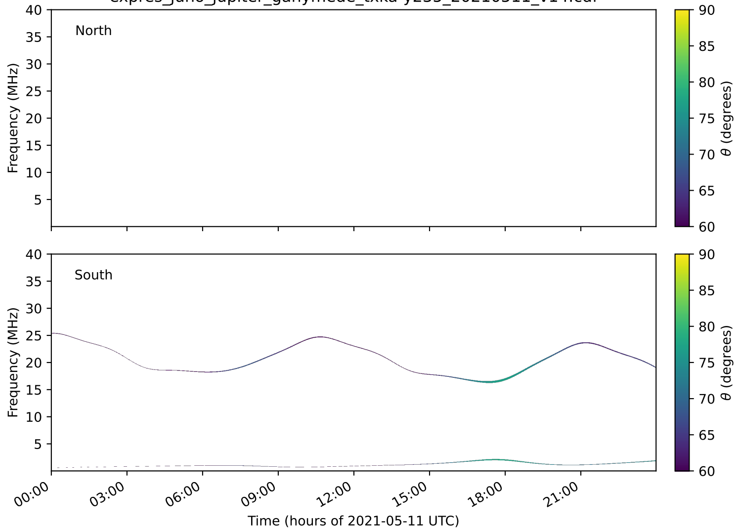
expres_juno_jupiter_ganymede_txka-y235_20210511_v14.cdf
