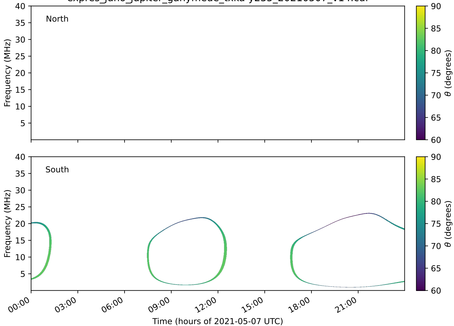
expres_juno_jupiter_ganymede_txka-y235_20210507_v14.cdf
