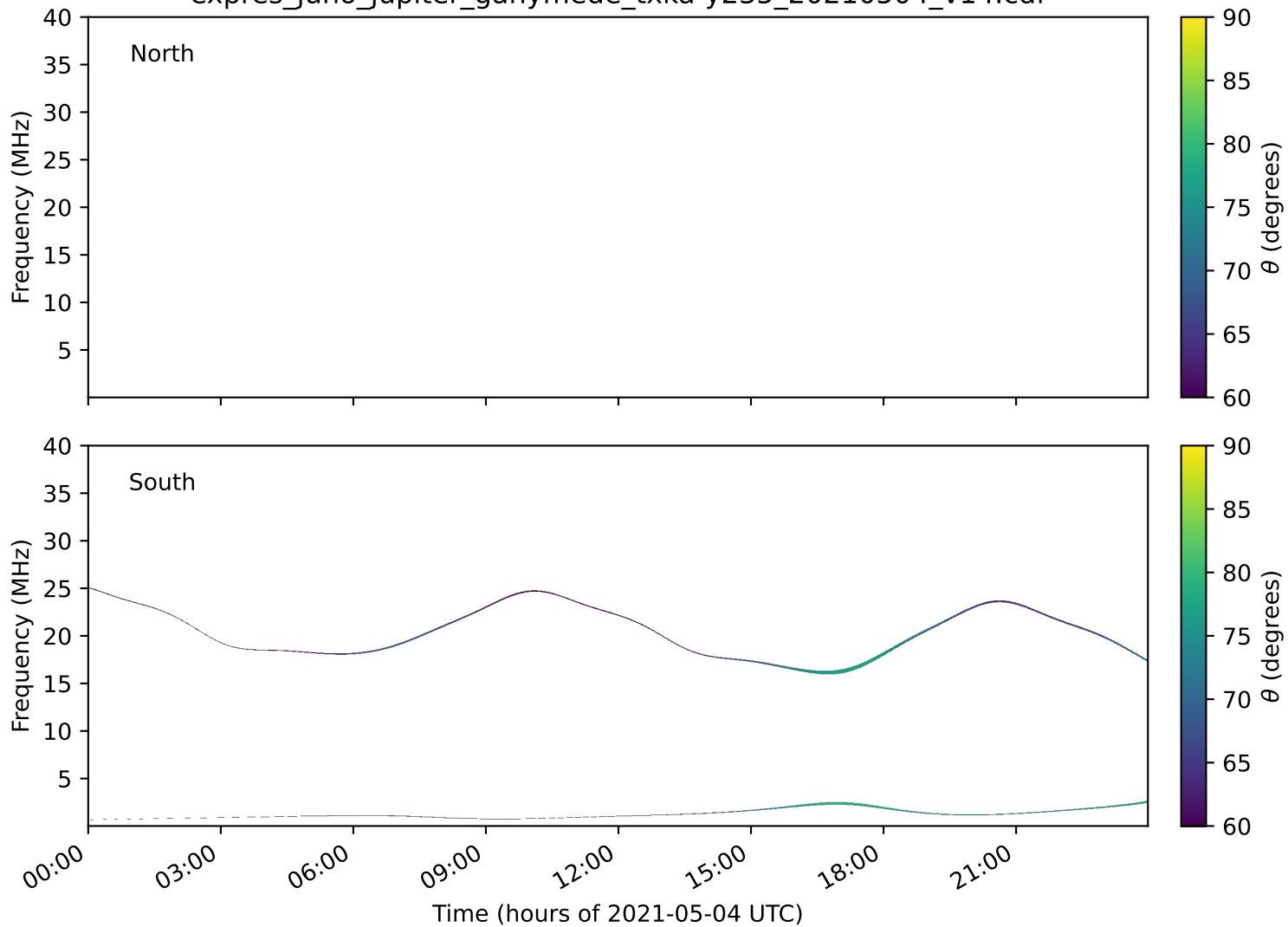
expres_juno_jupiter_ganymede_txka-y235_20210504_v14.cdf
