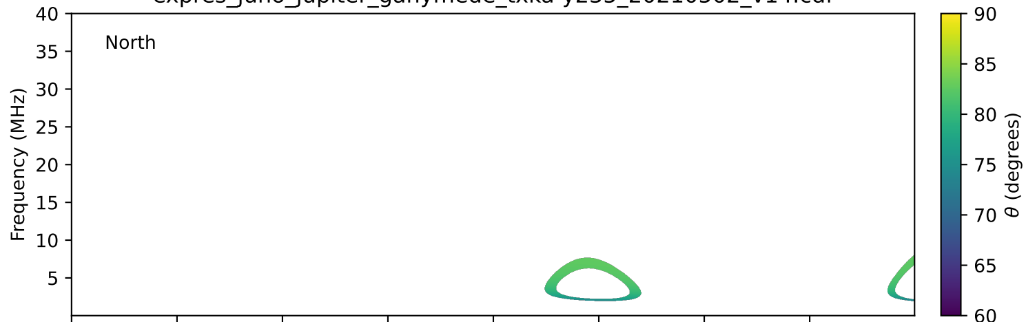
expres_juno_jupiter_ganymede_txka-y235_20210502_v14.cdf
