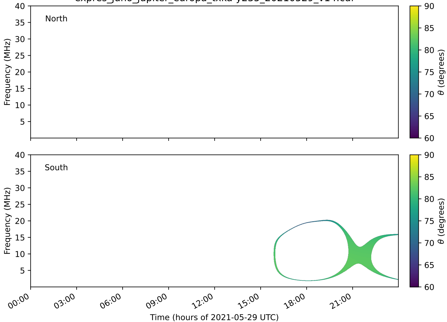
expres_juno_jupiter_europa_txka-y235_20210529_v14.cdf
