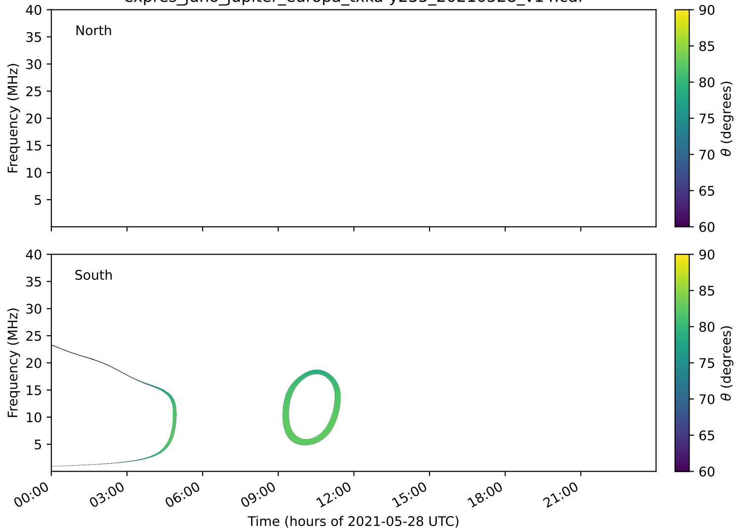
expres_juno_jupiter_europa_txka-y235_20210528_v14.cdf
